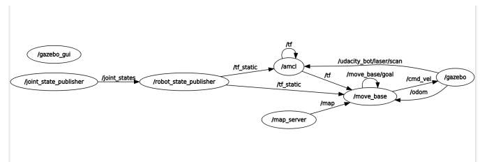
Fig. 8: Node relations
