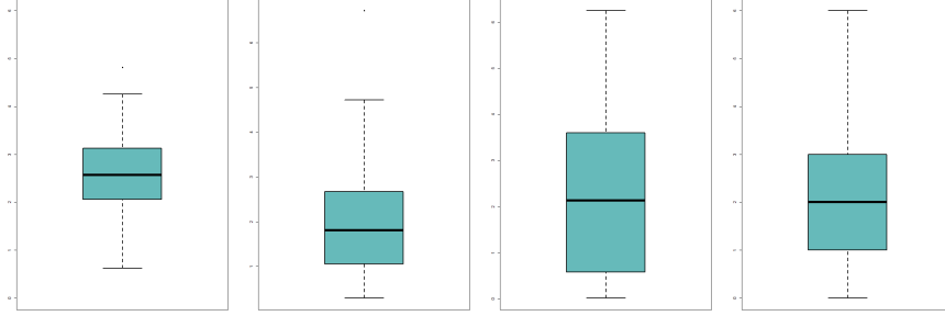
(b) Boxplot
